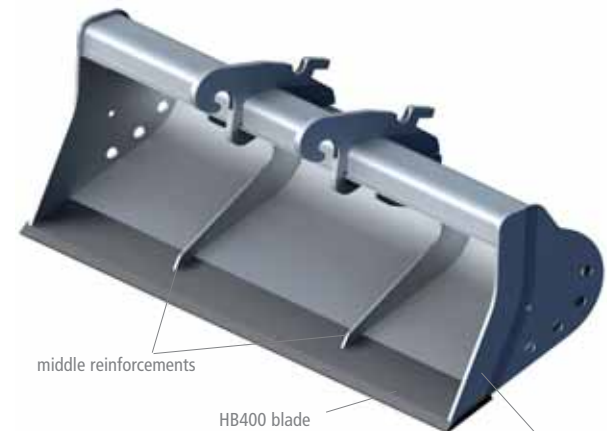
DC25 ditch cleaning bucket with anchoring for Verachtert CW quick coupler
